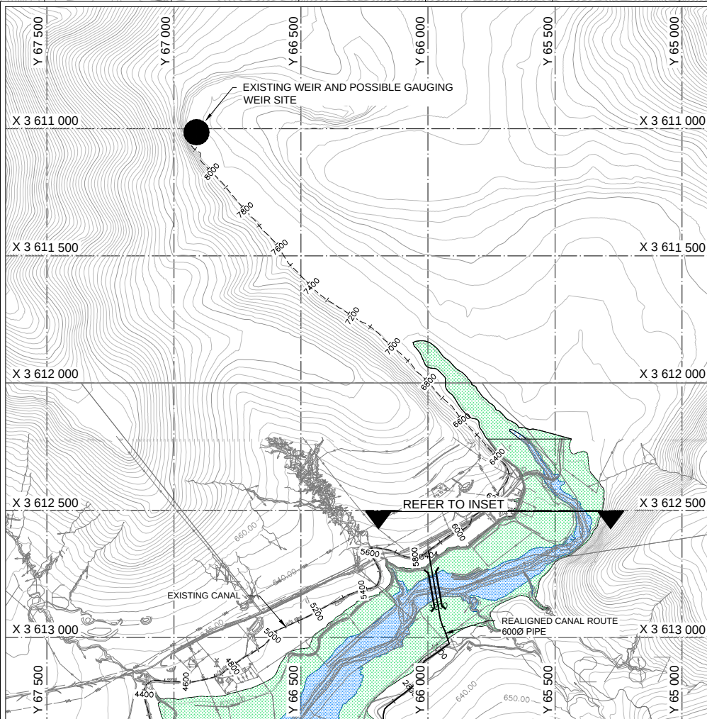
PLAN LAYOUT INSET SCALE 1:10 000
